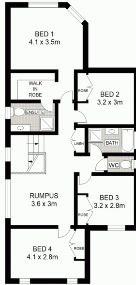
UPPER FLOOR
